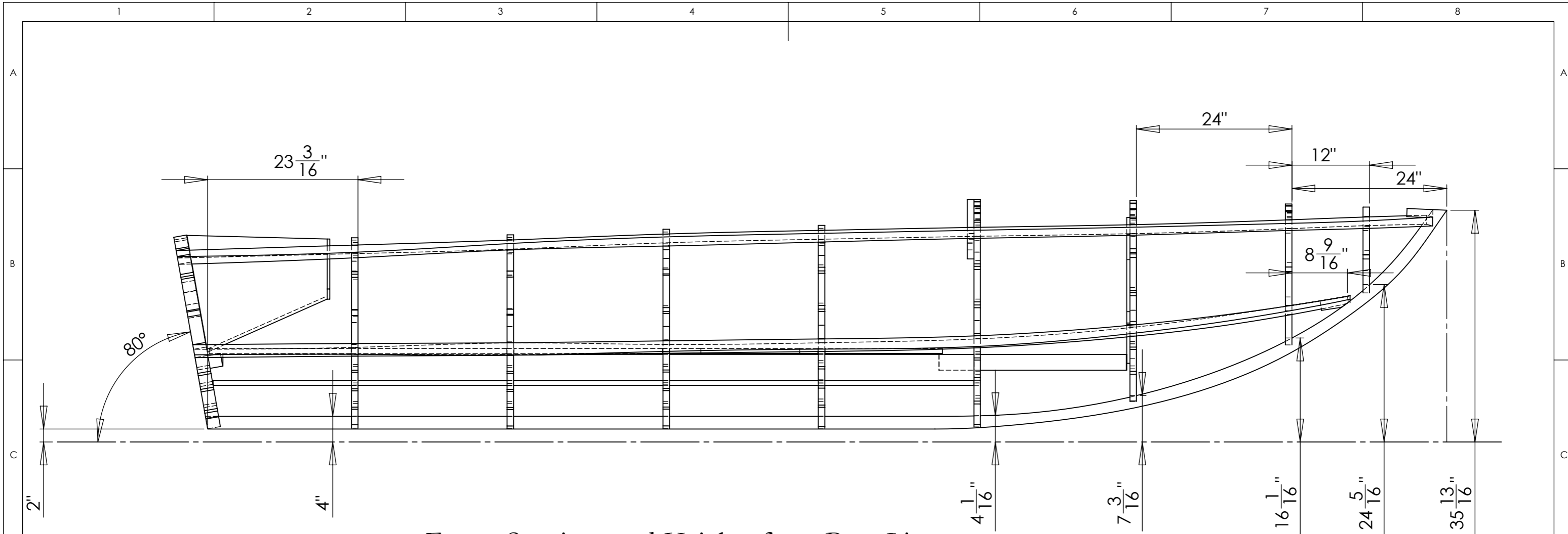
Frame Spacings and Heights from Base Line
